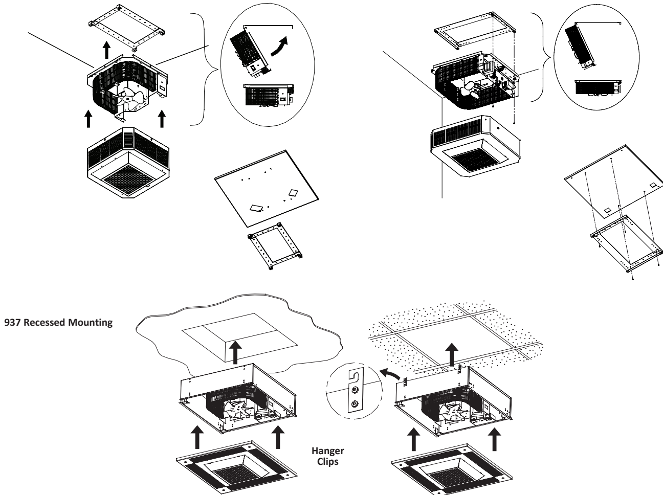
936 Surface Mounting for 2,000 to 5,000 Watt Heaters
