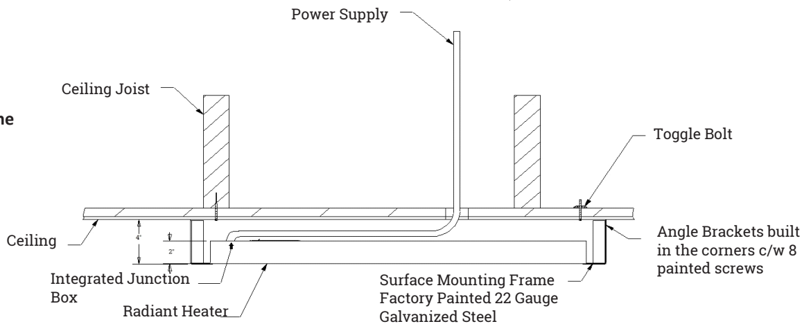
Cutaway View of AS Series
