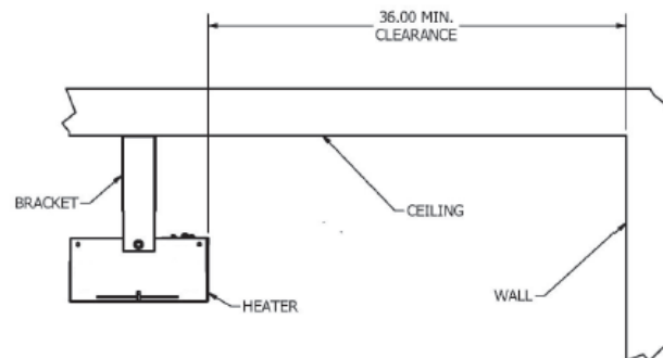
Fig. 2 – CEILING MOUNTING VERTICAL
