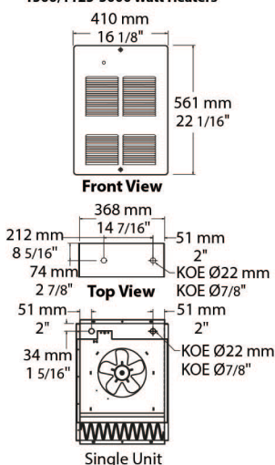
1500/1125-5000 Watt Heaters
