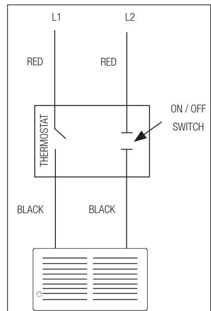
Double-pole Installation
