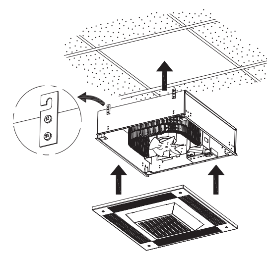
Fig. 2 Model (2 kW to 5 kW) Drop Ceiling Mounting
