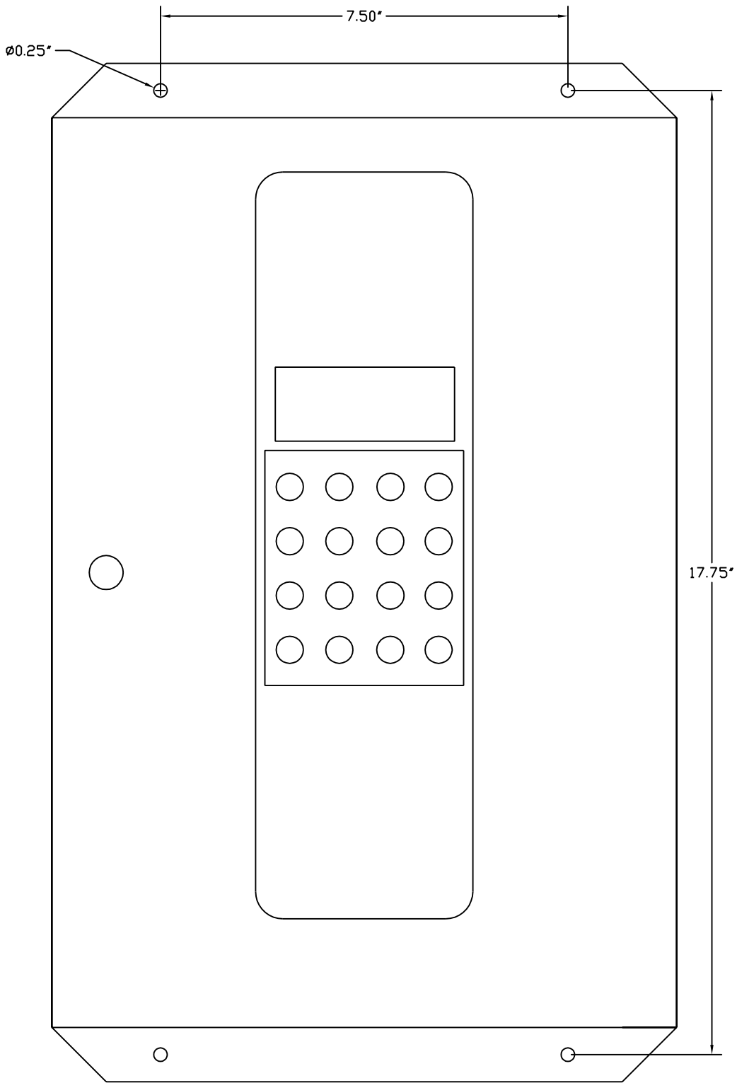
Brasch GDCP Control Panel Mounting Dimensions
